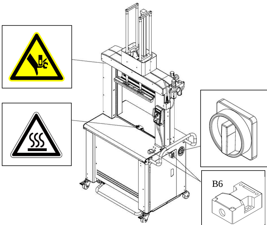
For TP-702P-59
