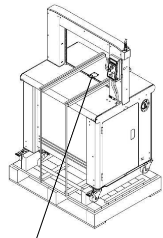
Center-of-gravity position
