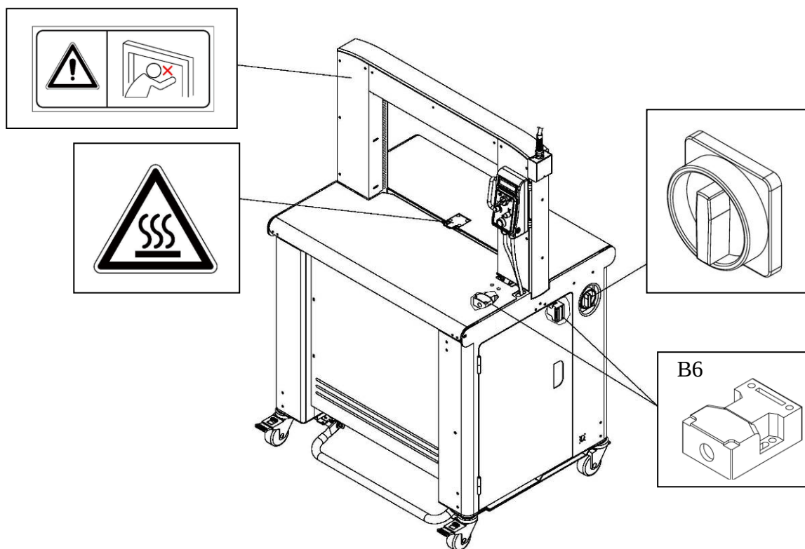
For TP-702RS
